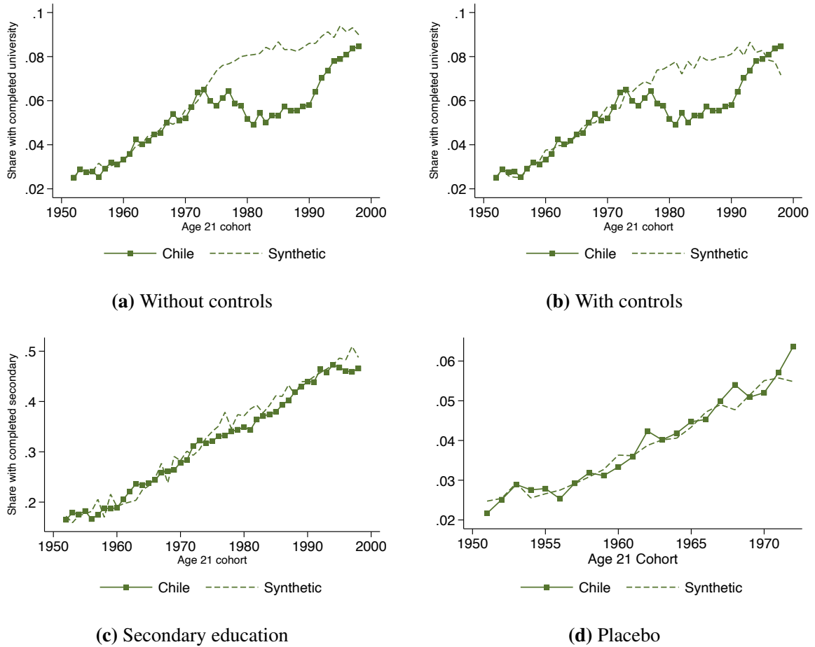
Figure 5: Synthetic control
